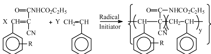
Sch. 1. Copolymer synthesis (where R is 4-CH 3 CH 2 , 4-(CH 3 ) 2 CH, 4-CH 3 (CH 2 ) 3 , 2,4-(CH 3 ) 2 , 2,5-(CH 3 ) 2 , 2-C 2 H 5 O, 3-C 2 H 5 O, 4-CH 3 (CH 2 ) 2 O, 4-CH 3 (CH 2 ) 3 O, and 4-CH 3 (CH 2 ) 5 O).
